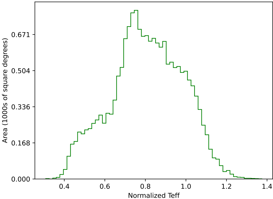
smc_lmc_v3.3_10yrs WFD g band: Normalized Teff
