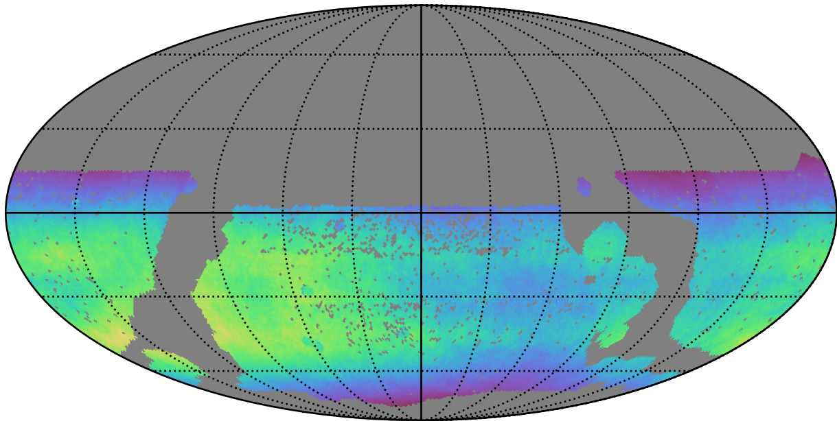
smc_lmc_v3.3_10yrs WFD all bands: Normalized Teff
