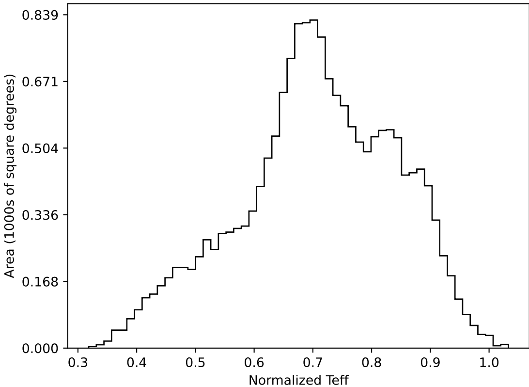
smc_lmc_v3.3_10yrs WFD all bands: Normalized Teff
