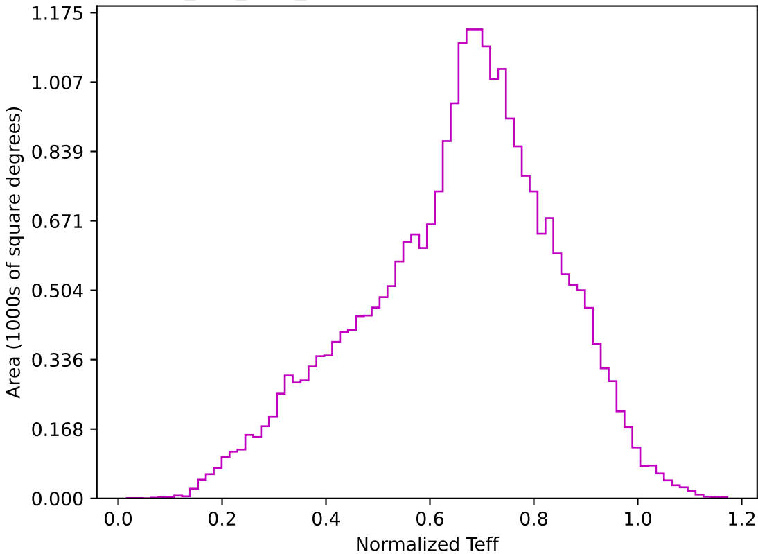
smc_lmc_v3.3_10yrs All sky z band: Normalized Teff
