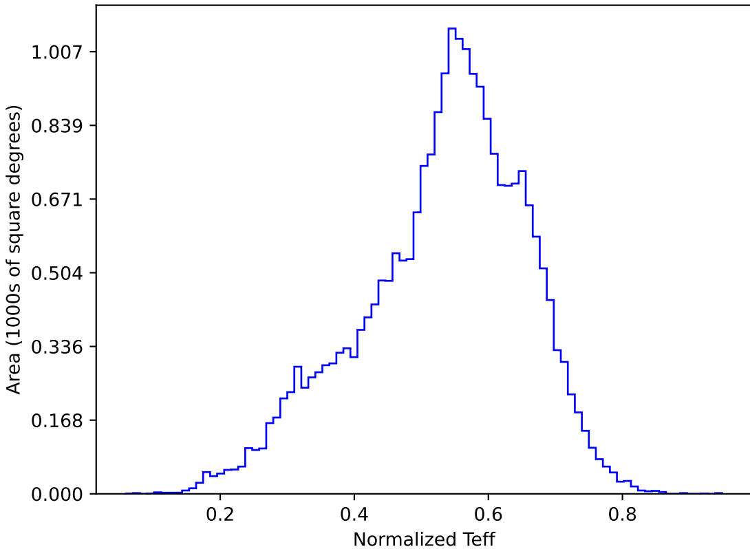
smc_lmc_v3.3_10yrs All sky y band: Normalized Teff
