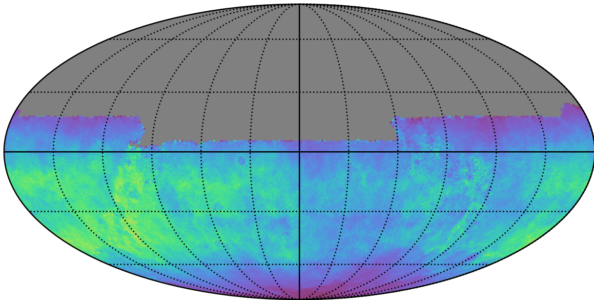
smc_lmc_v3.3_10yrs All sky u band: Normalized Teff
