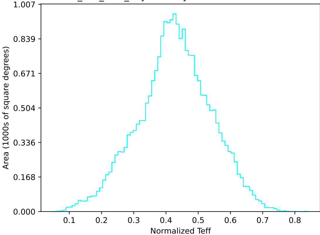
smc_lmc_v3.3_10yrs All sky u band: Normalized Teff
