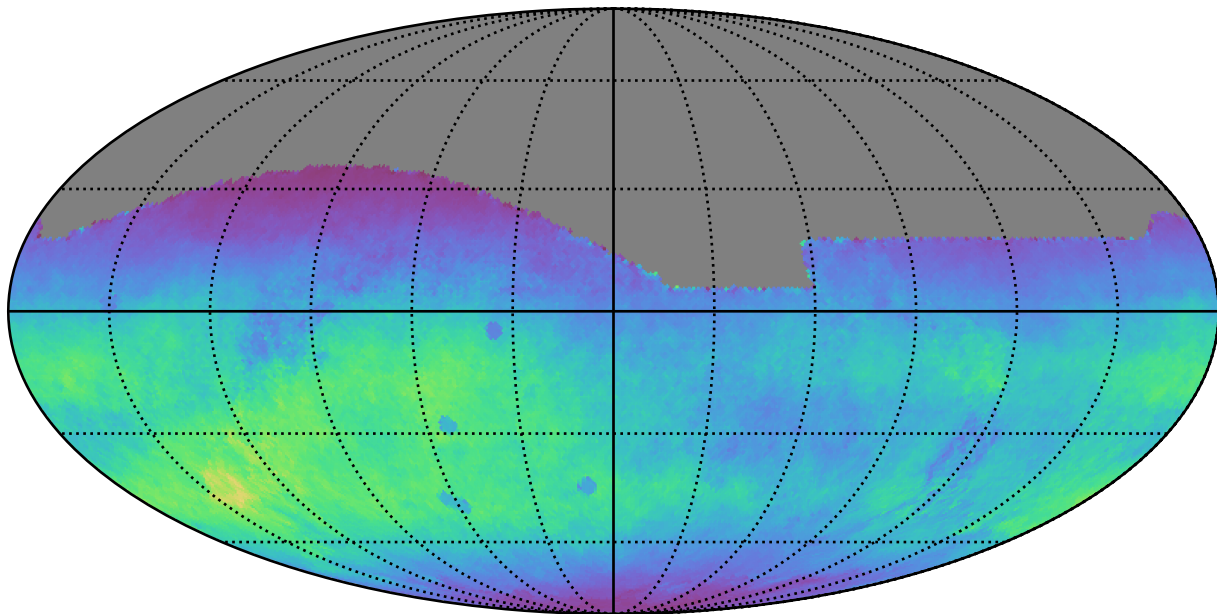
smc_lmc_v3.3_10yrs All sky r band: Normalized Teff
