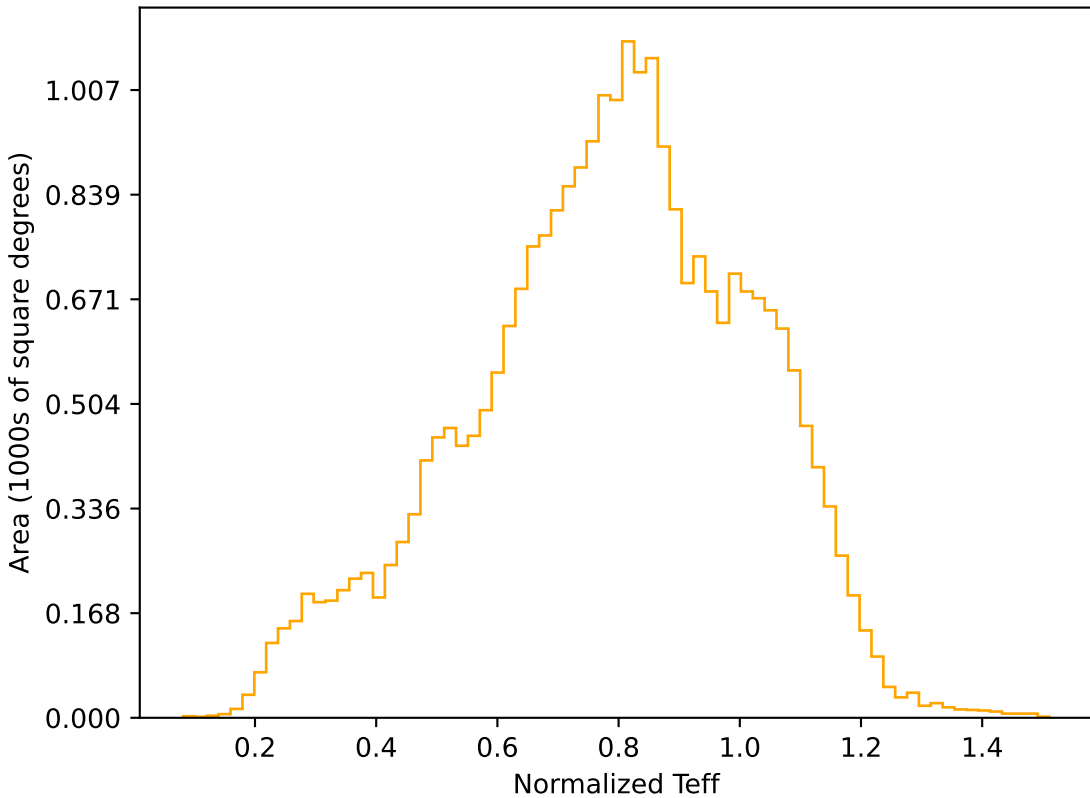
smc_lmc_v3.3_10yrs All sky r band: Normalized Teff
