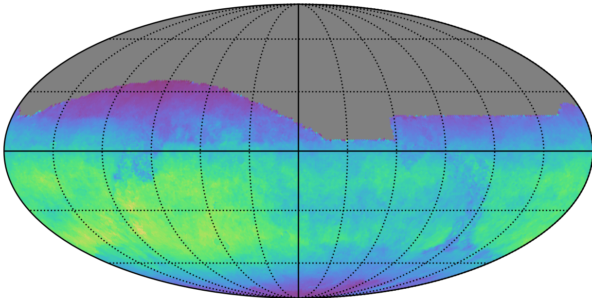
smc_lmc_v3.3_10yrs All sky i band: Normalized Teff
