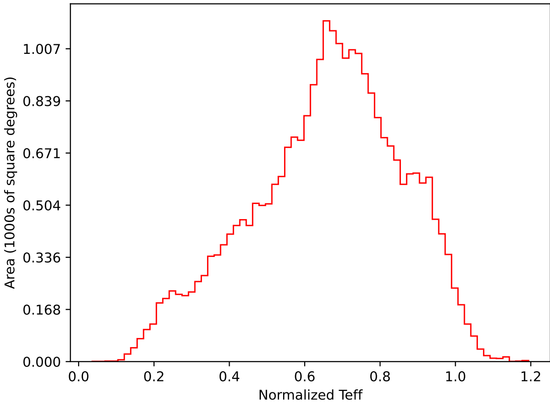
smc_lmc_v3.3_10yrs All sky i band: Normalized Teff
