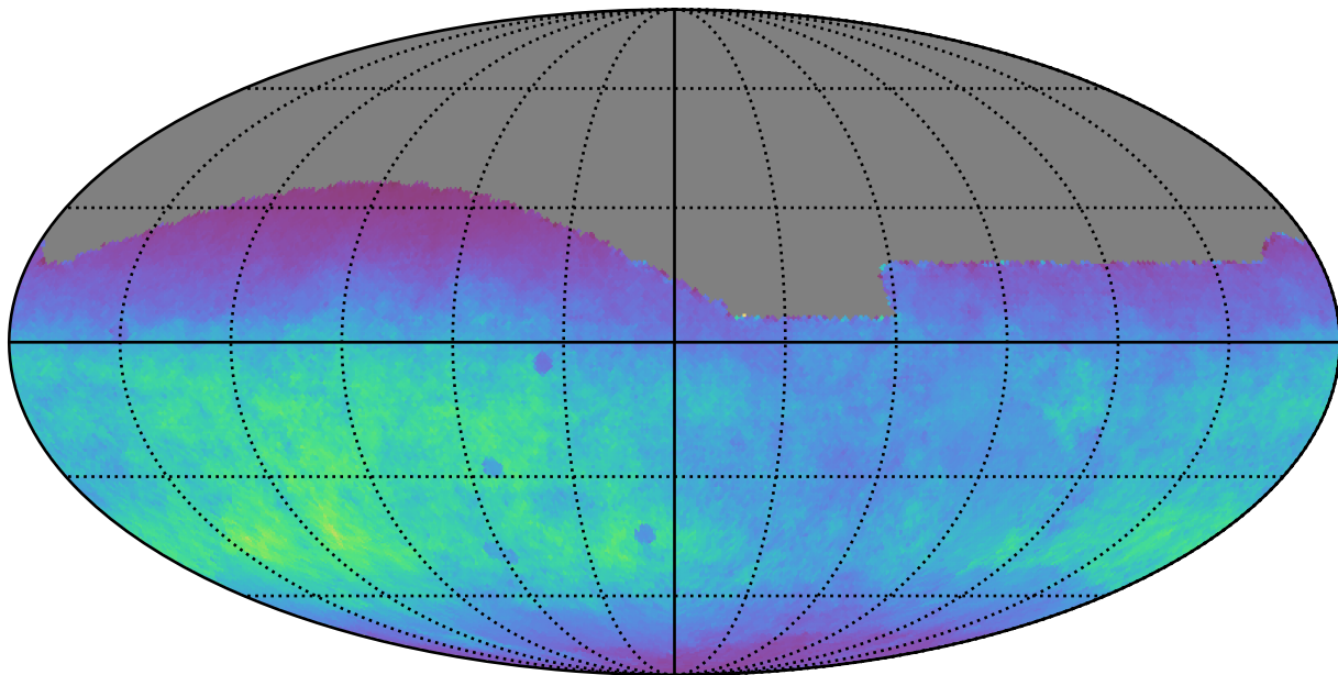
smc_lmc_v3.3_10yrs All sky g band: Normalized Teff
