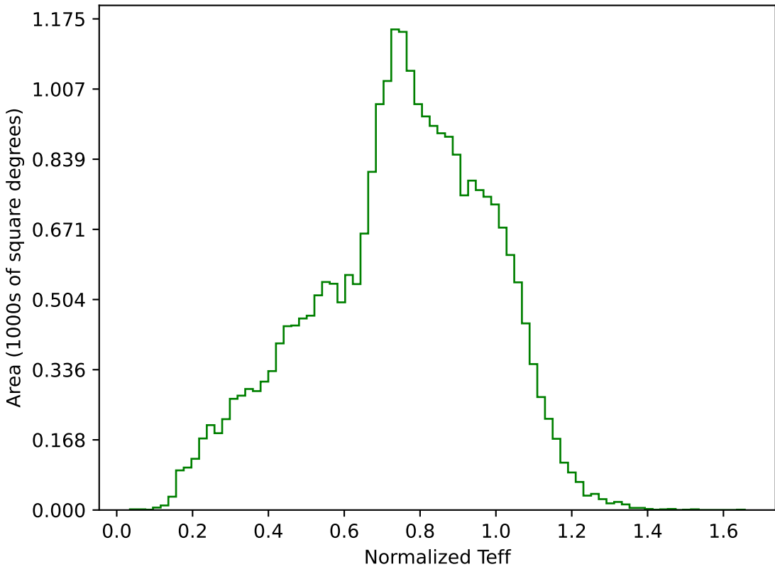
smc_lmc_v3.3_10yrs All sky g band: Normalized Teff
