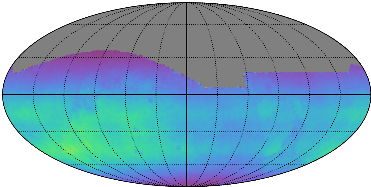
smc_lmc_v3.3_10yrs All sky all bands: Normalized Teff
