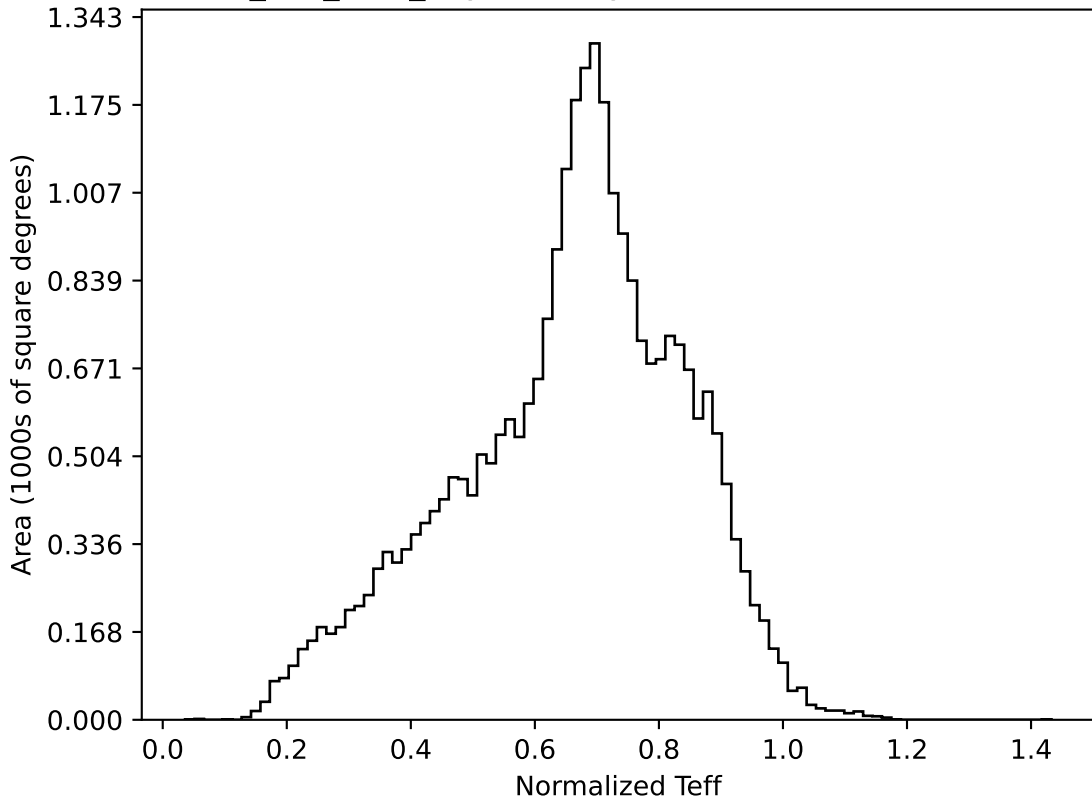
smc_lmc_v3.3_10yrs All sky all bands: Normalized Teff
