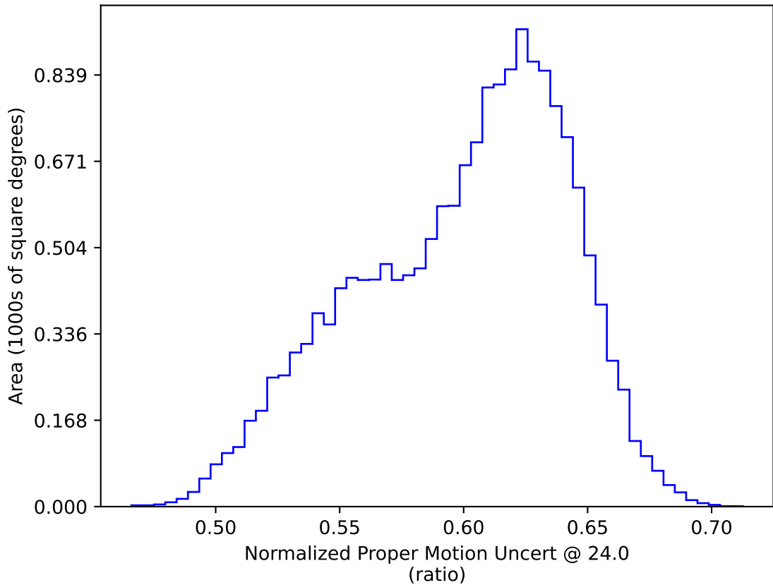
smc_lmc_v3.3_10yrs WFD: Normalized Proper Motion Uncert @ 24.0
