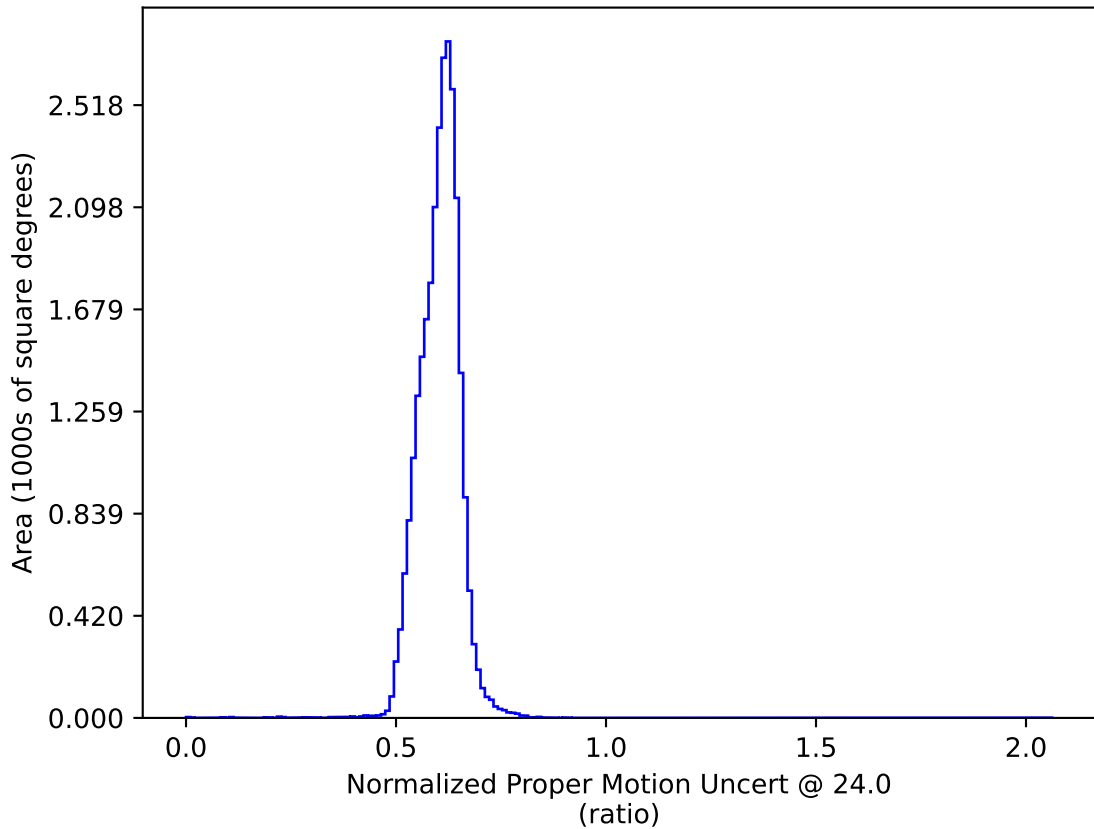
smc_lmc_v3.3_10yrs All sky: Normalized Proper Motion Uncert @ 24.0
