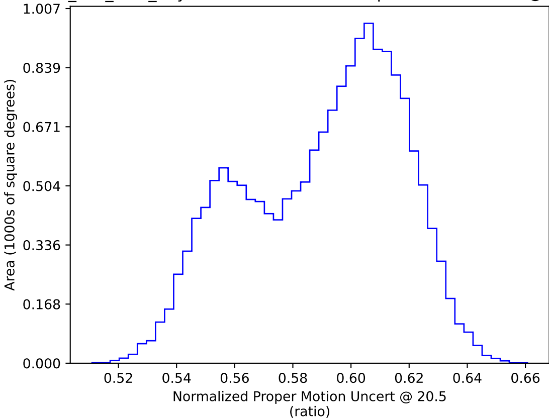
smc_lmc_v3.3_10yrs WFD: Normalized Proper Motion Uncert @ 20.5
