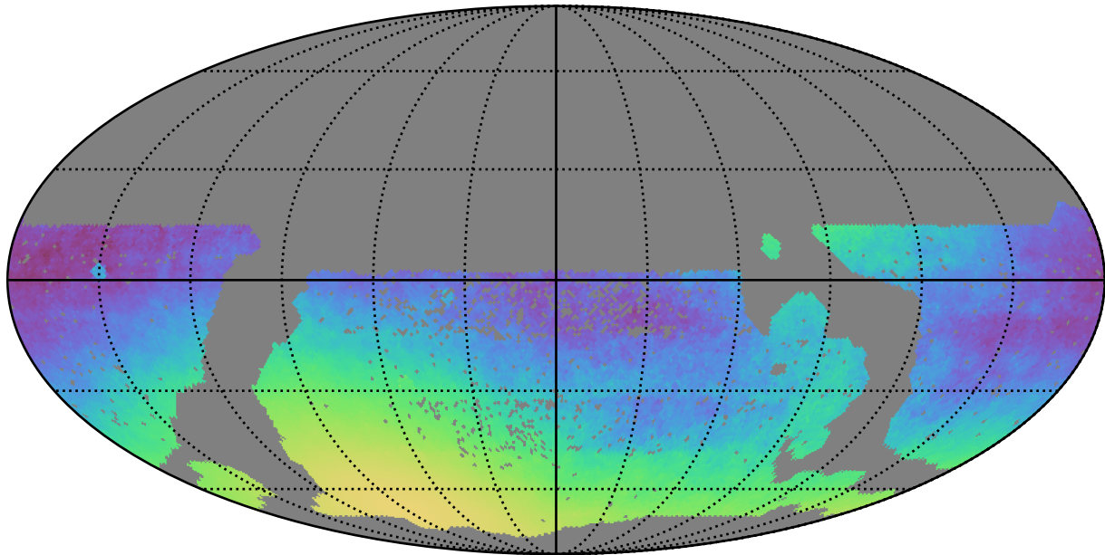
smc_lmc_v3.3_10yrs WFD: Normalized Parallax Uncert @ 24.0
