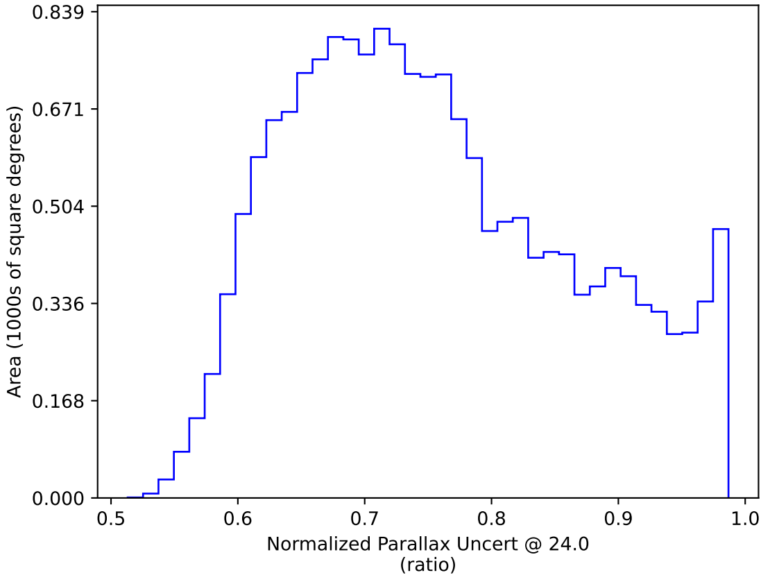
smc_lmc_v3.3_10yrs WFD: Normalized Parallax Uncert @ 24.0
