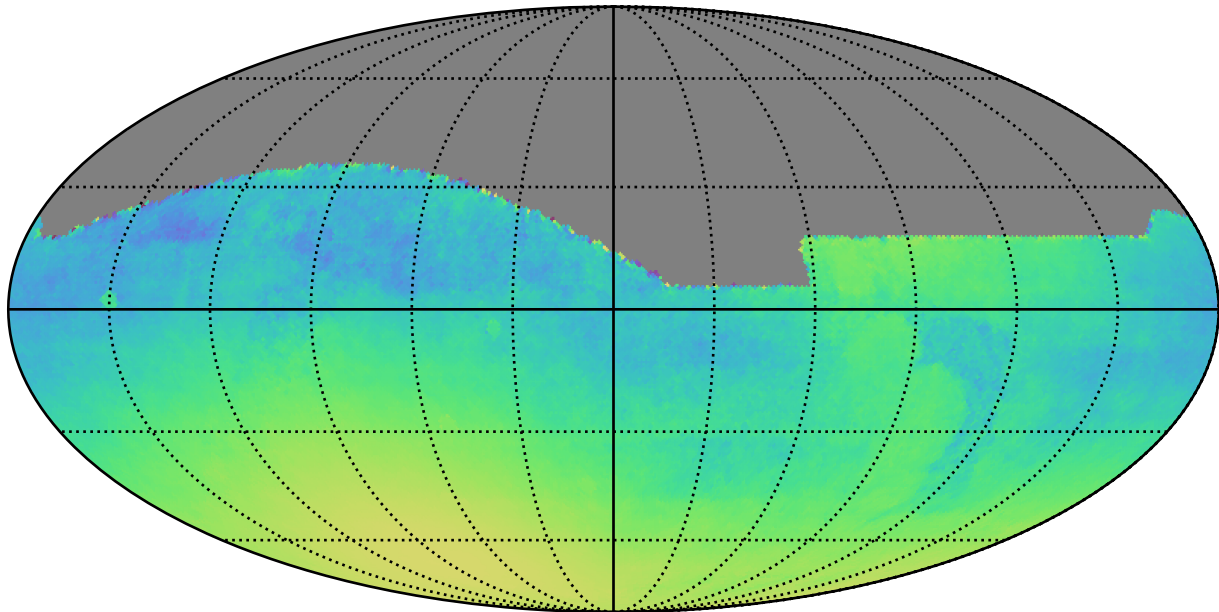
smc_lmc_v3.3_10yrs All sky: Normalized Parallax Uncert @ 24.0
