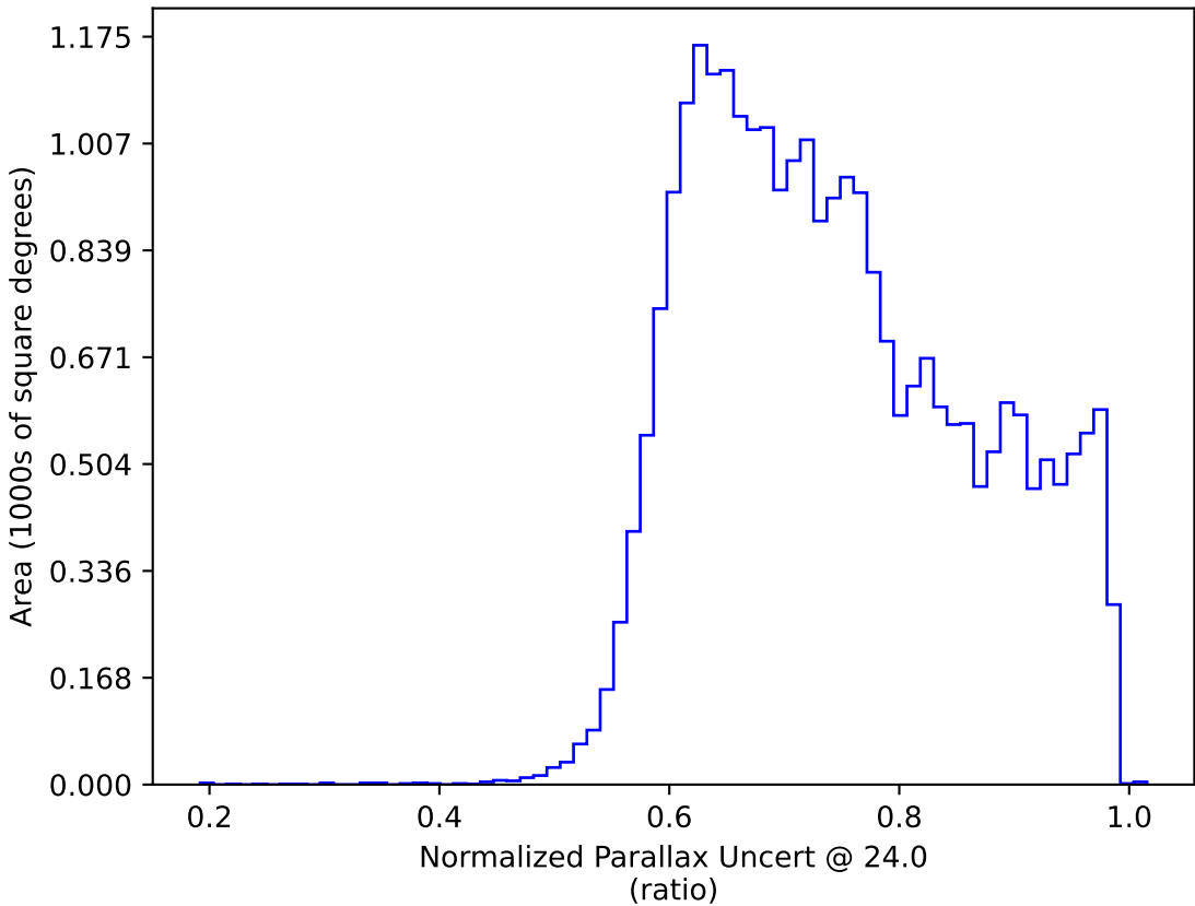
smc_lmc_v3.3_10yrs All sky: Normalized Parallax Uncert @ 24.0
