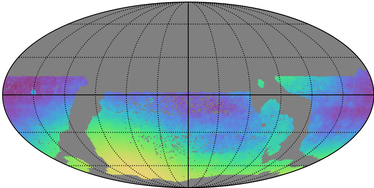
smc_lmc_v3.3_10yrs WFD: Normalized Parallax Uncert @ 22.4
