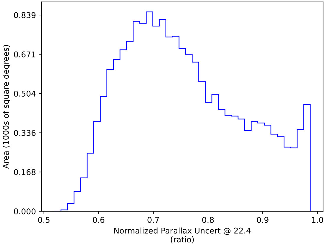
smc_lmc_v3.3_10yrs WFD: Normalized Parallax Uncert @ 22.4
