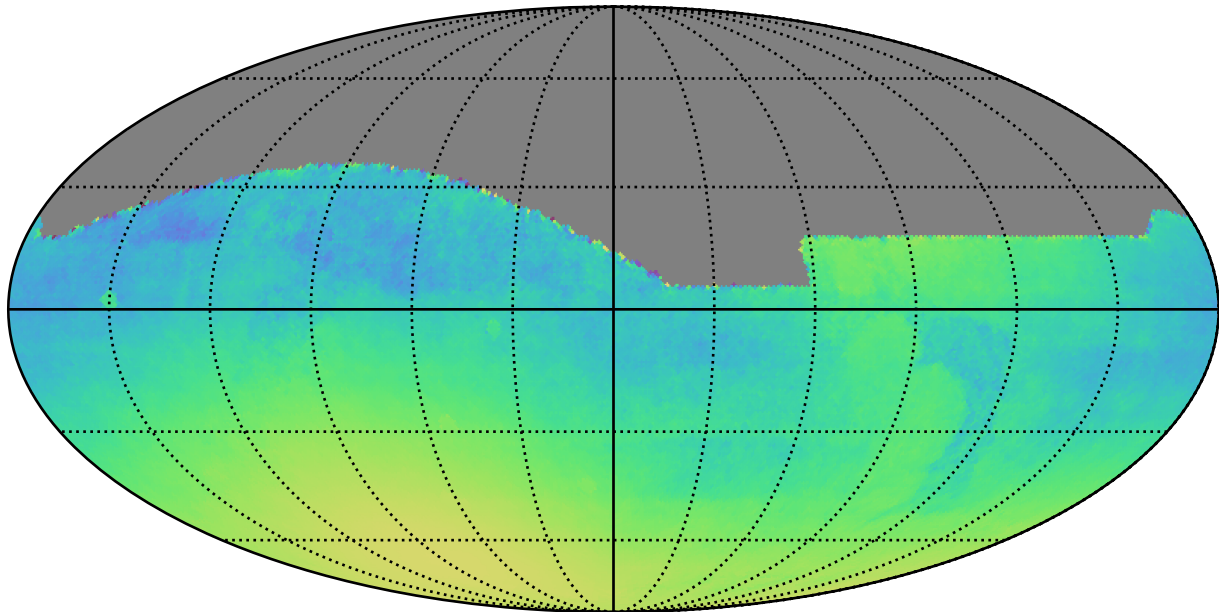
smc_lmc_v3.3_10yrs All sky: Normalized Parallax Uncert @ 22.4
