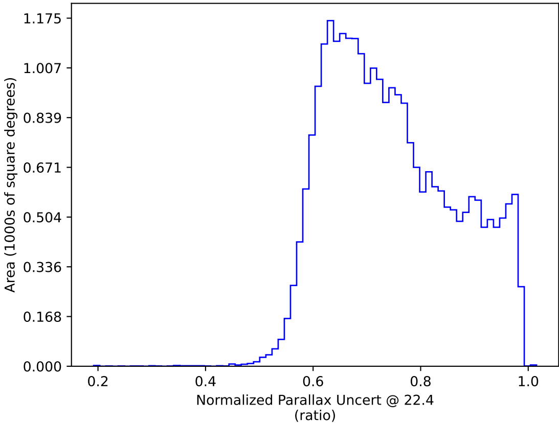
smc_lmc_v3.3_10yrs All sky: Normalized Parallax Uncert @ 22.4
