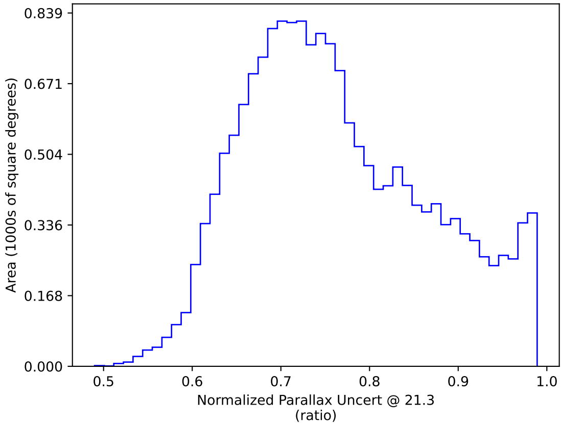
smc_lmc_v3.3_10yrs WFD y band only: Normalized Parallax Uncert @ 21.3
