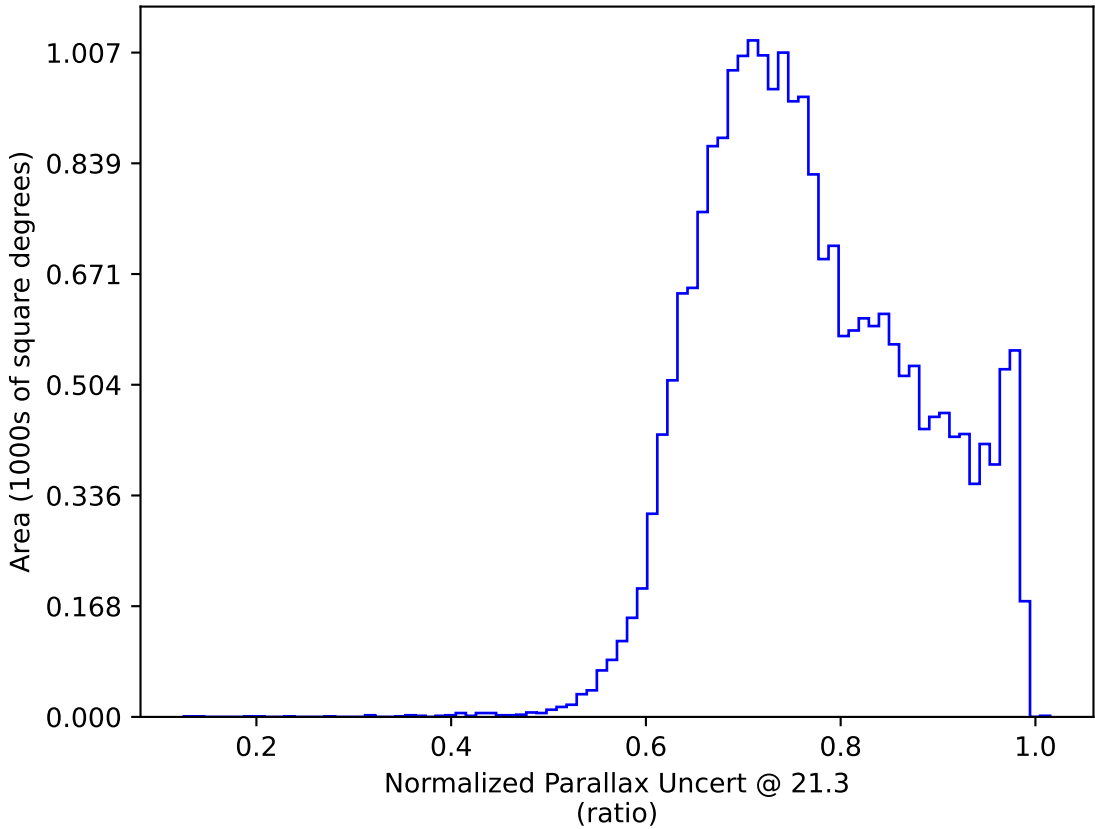
smc_lmc_v3.3_10yrs All sky y band only: Normalized Parallax Uncert @ 21.3
