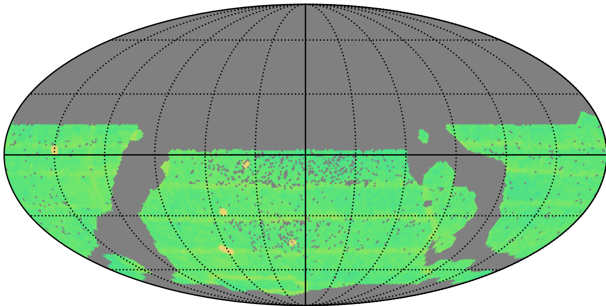
smc_lmc_v3.3_10yrs WFD all bands: N Unique Nights
