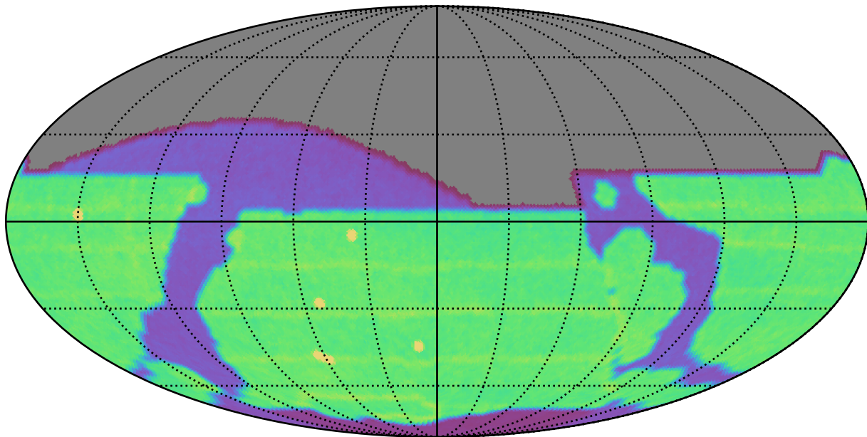
smc_lmc_v3.3_10yrs All sky all bands: N Unique Nights
