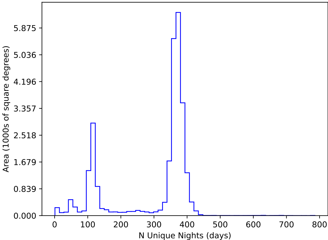
smc_lmc_v3.3_10yrs All sky all bands: N Unique Nights
