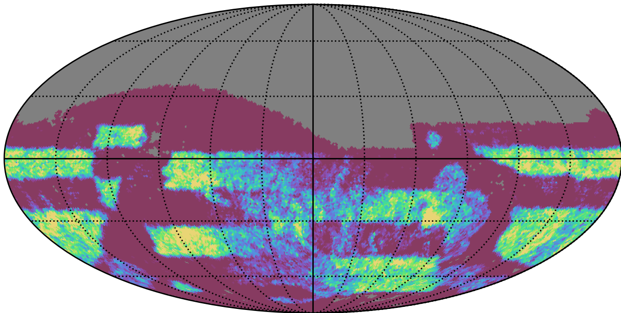
smc_lmc_v3.3_10yrs Yr 3-4 z band: NVisits
