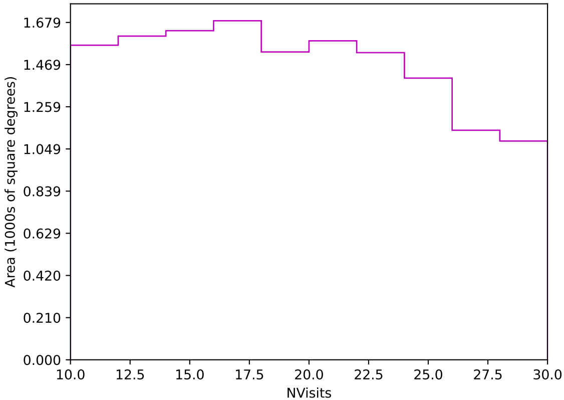
smc_lmc_v3.3_10yrs Yr 3-4 z band: NVisits
