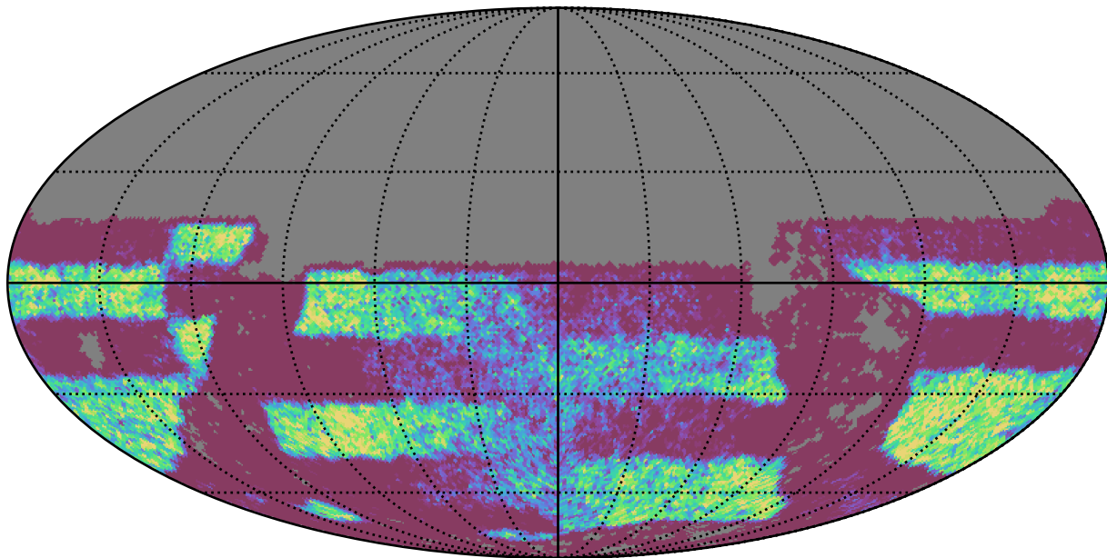
smc_lmc_v3.3_10yrs Yr 3-4 y band: NVisits
