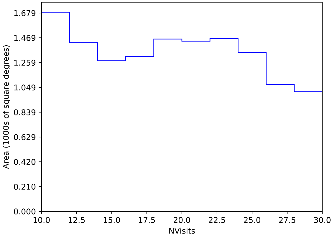
smc_lmc_v3.3_10yrs Yr 3-4 y band: NVisits
