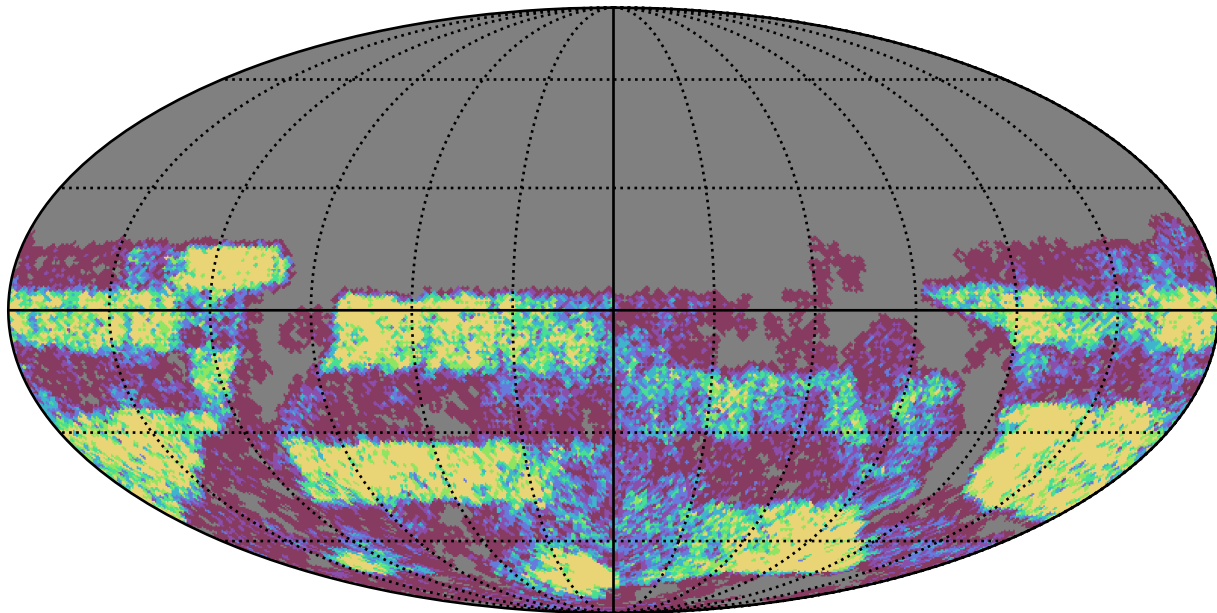
smc_lmc_v3.3_10yrs Yr 3-4 u band: NVisits
