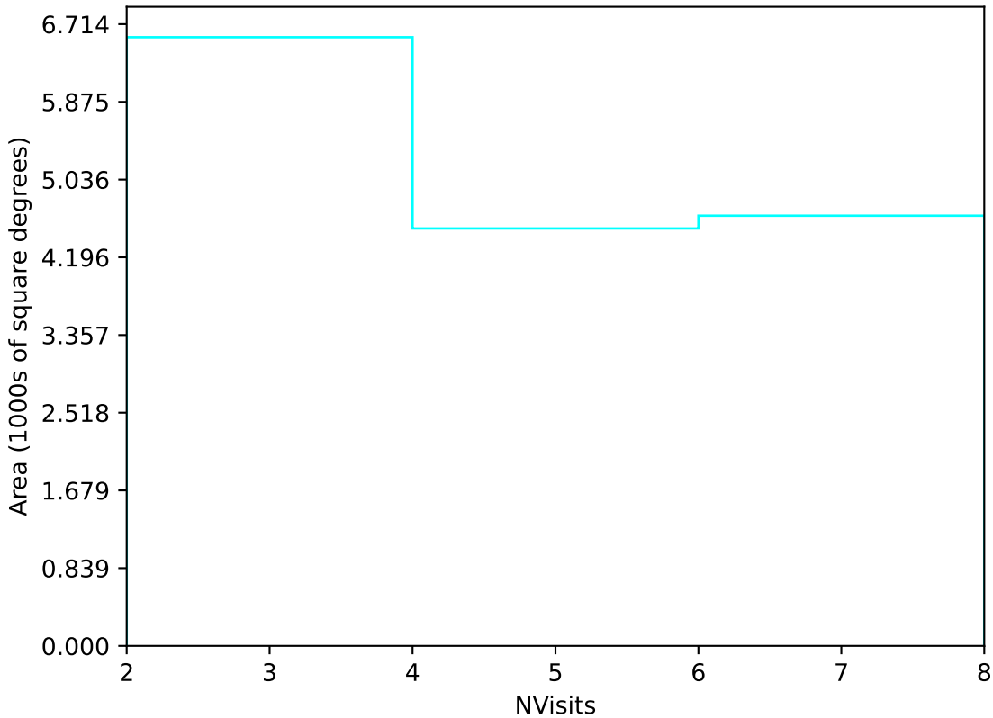
smc_lmc_v3.3_10yrs Yr 3-4 u band: NVisits
