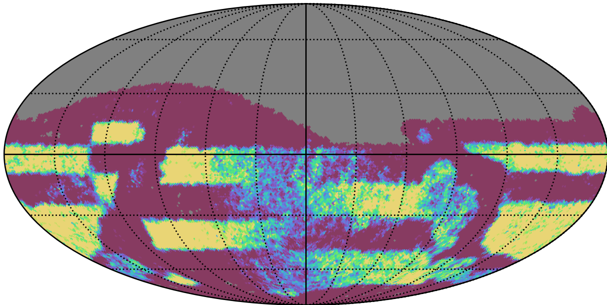
smc_lmc_v3.3_10yrs Yr 3-4 r band: NVisits
