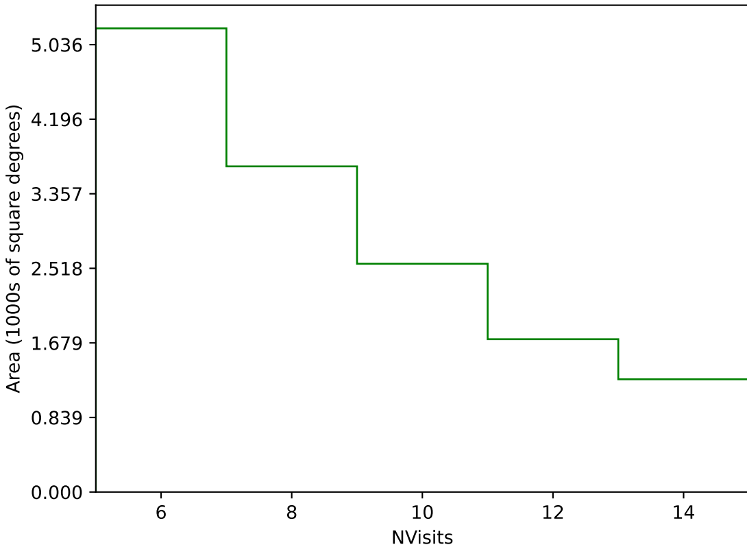
smc_lmc_v3.3_10yrs Yr 3-4 g band: NVisits
