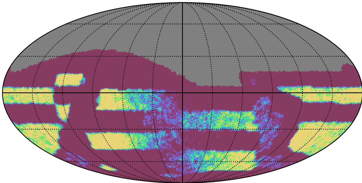
smc_lmc_v3.3_10yrs Yr 3-4 all bands: NVisits
