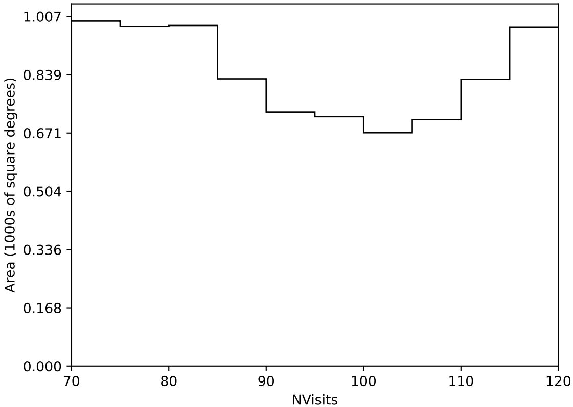
smc_lmc_v3.3_10yrs Yr 3-4 all bands: NVisits
