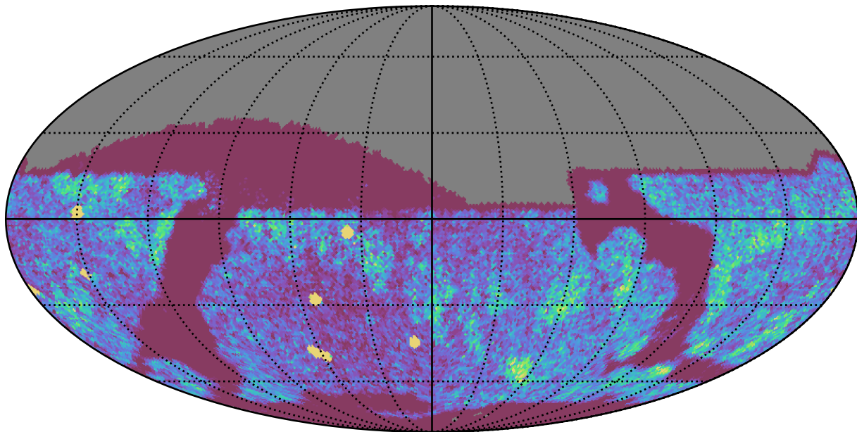
smc_lmc_v3.3_10yrs Yr 1 z band: NVisits
