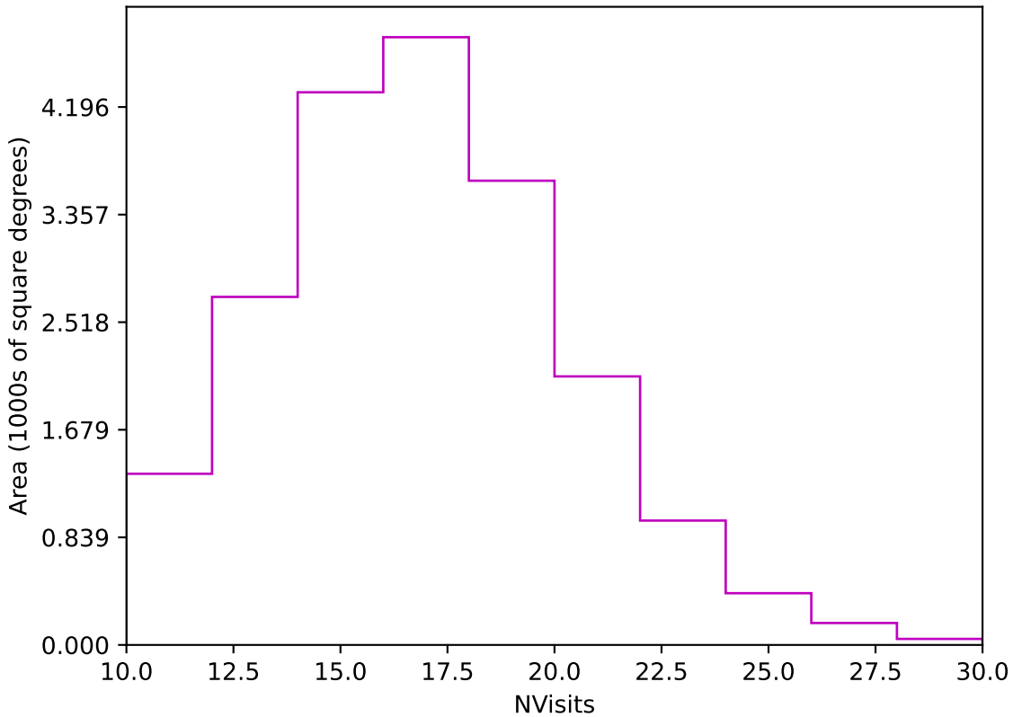
smc_lmc_v3.3_10yrs Yr 1 z band: NVisits
