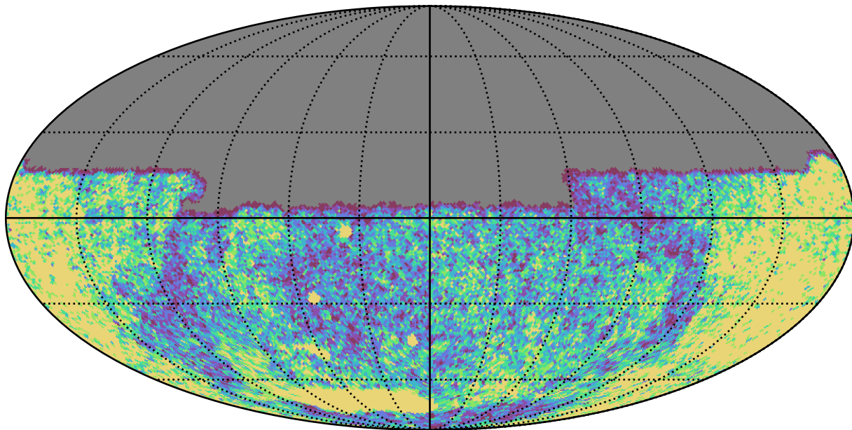
smc_lmc_v3.3_10yrs Yr 1 u band: NVisits
