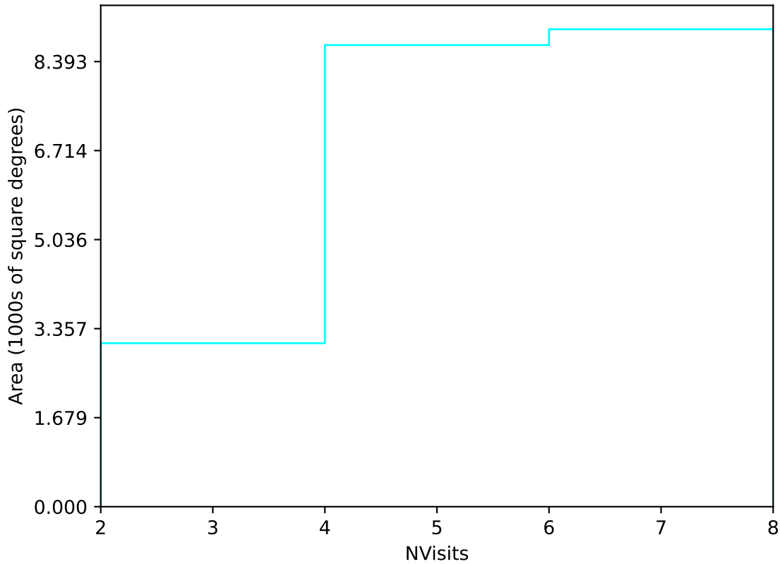
smc_lmc_v3.3_10yrs Yr 1 u band: NVisits
