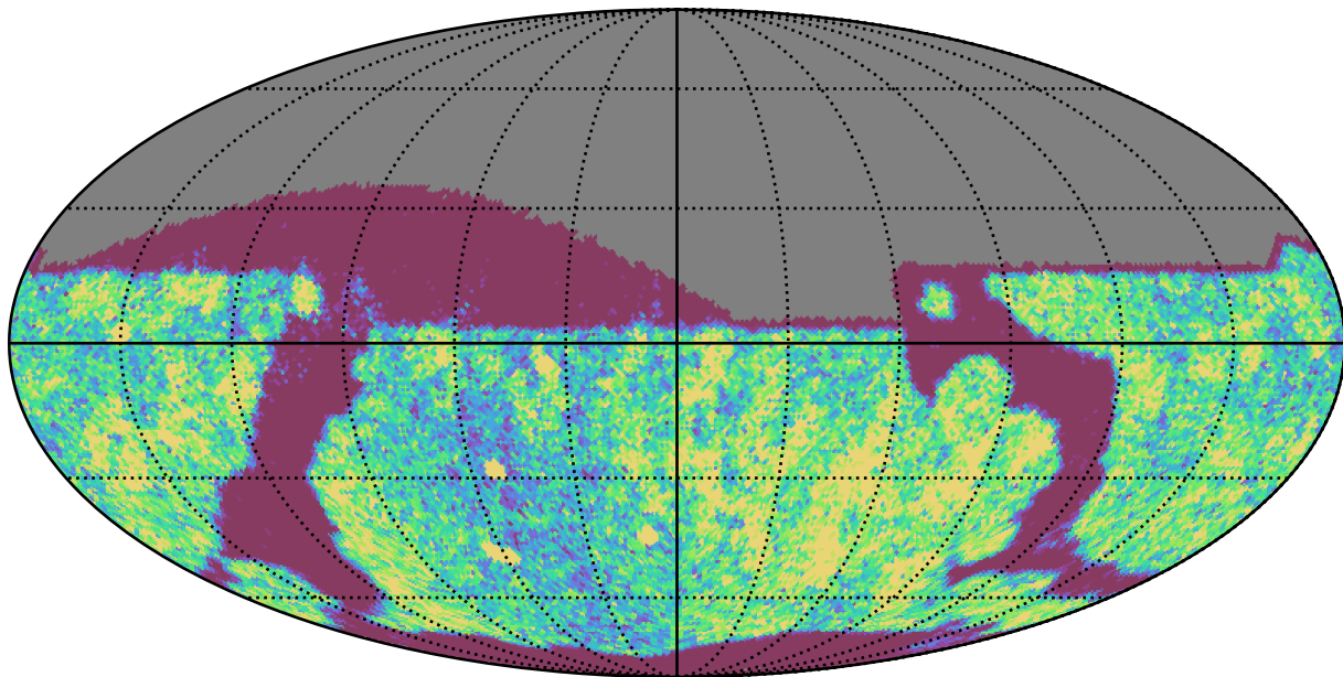
smc_lmc_v3.3_10yrs Yr 1 i band: NVisits
