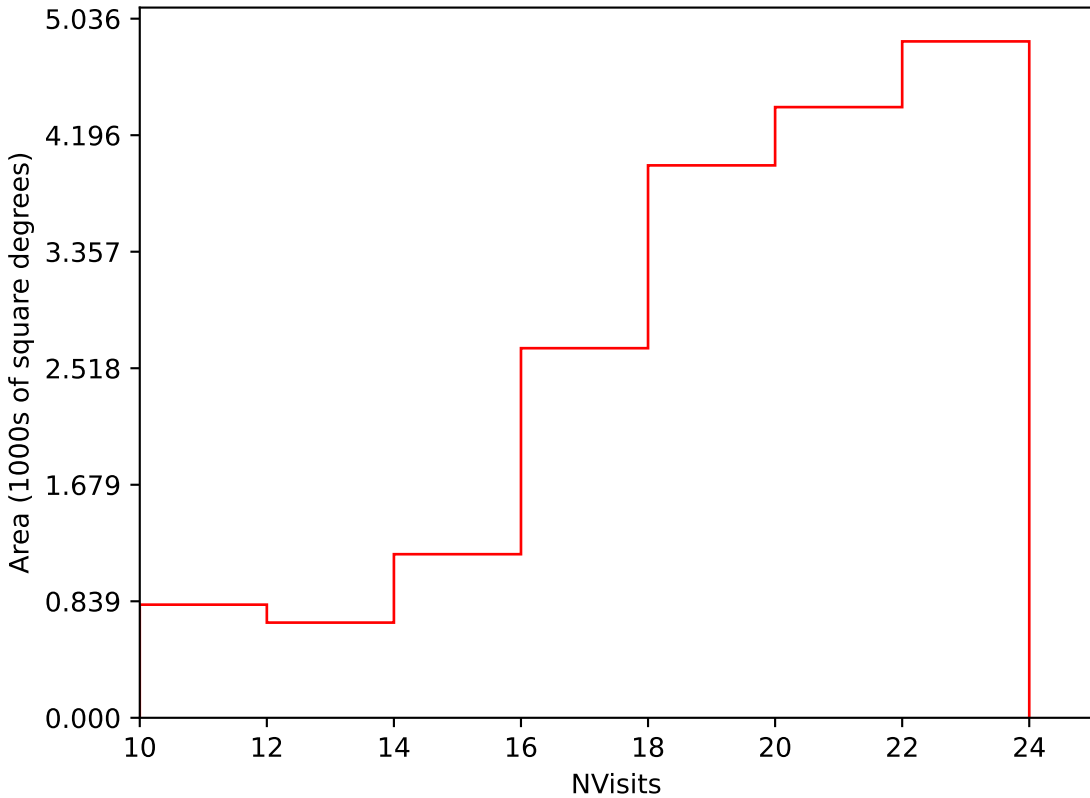
smc_lmc_v3.3_10yrs Yr 1 i band: NVisits
