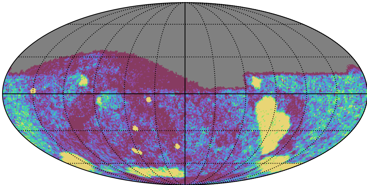
smc_lmc_v3.3_10yrs Yr 1 g band: NVisits
