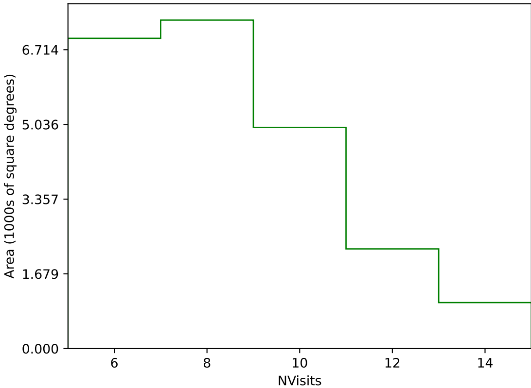
smc_lmc_v3.3_10yrs Yr 1 g band: NVisits
