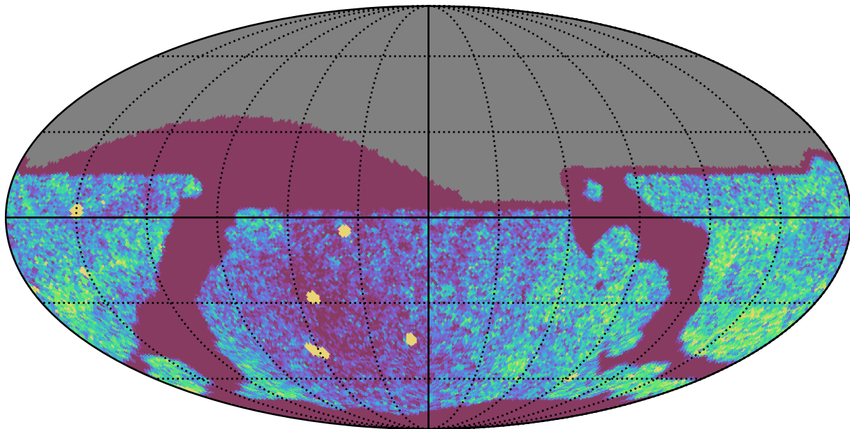
smc_lmc_v3.3_10yrs Yr 1 all bands: NVisits
